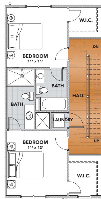
UPPER FLOOR
