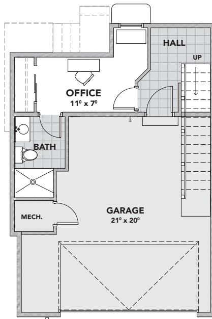
LOWER LEVEL/GARAGE
