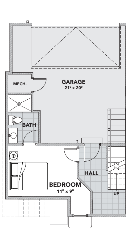
LOWER LEVEL/GARAGE
