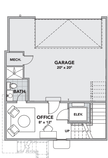
LOWER LEVEL/GARAGE
